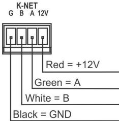
Figure 4: K-NET PINOUT Connection
