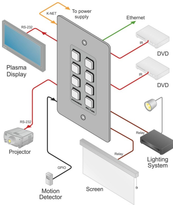
Figure 3: Connecting the RC-76R/RC-78R Room Controllers
