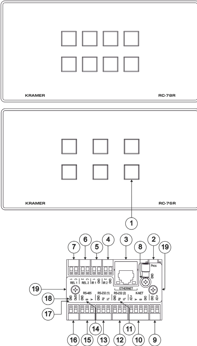
Figure 2: RC-76R/RC-78R Room Controllers – EU / UK Size
