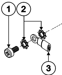
Figure 5: Grounding Connection Components
