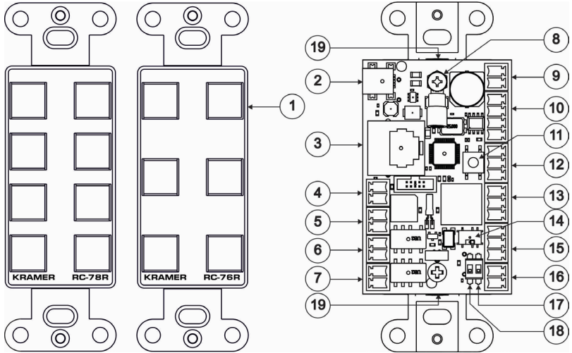
Figure 1: RC-76R/RC-78R Room Controllers – US-D Size
